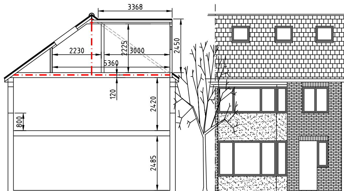
Front 1:100
