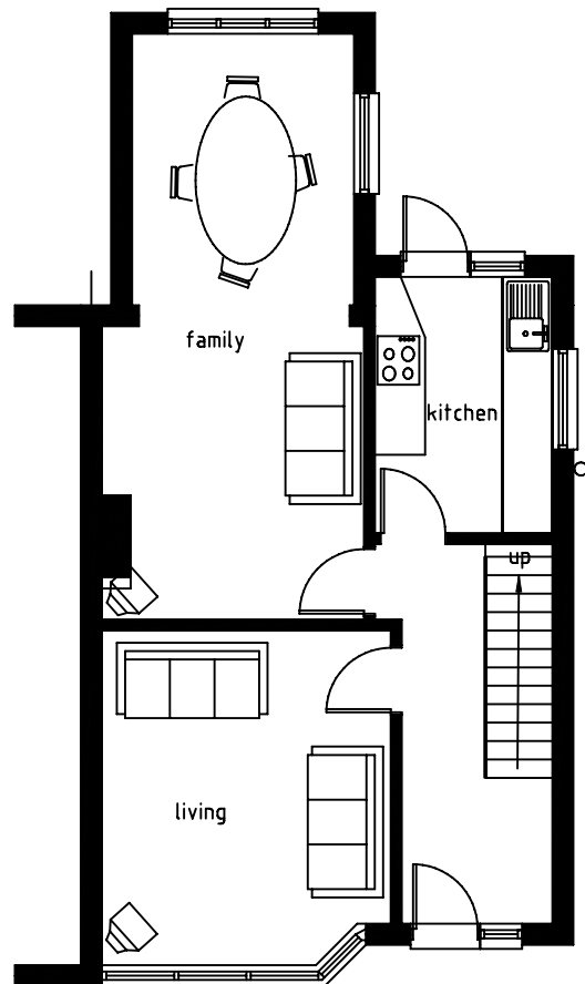
Ground 1:100
