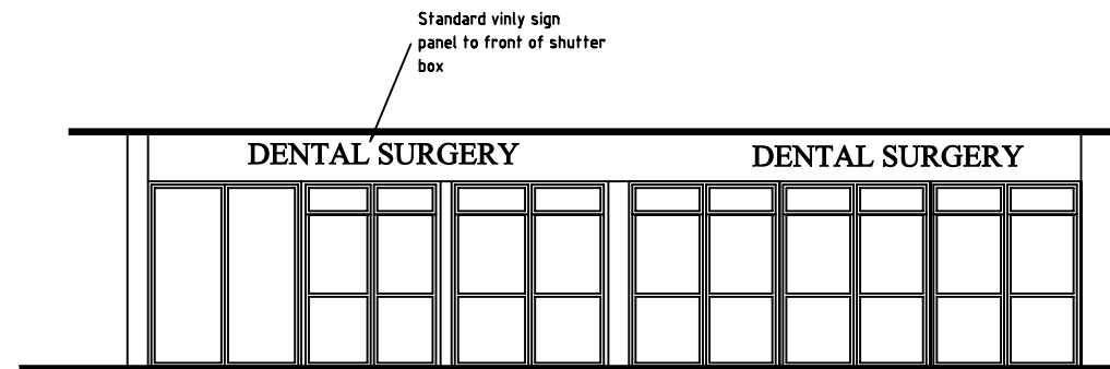
Front 1:100
